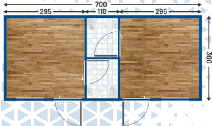
Model K-114
