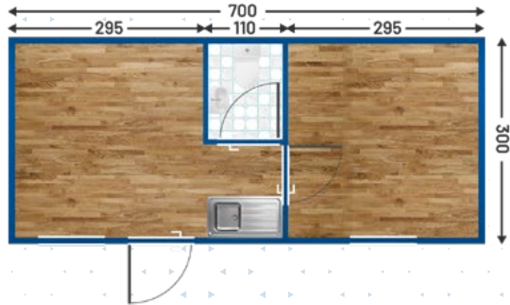
Model K-111
