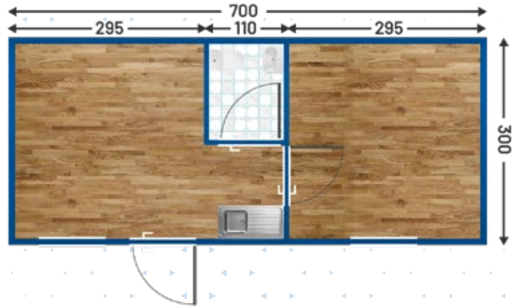
Model K-113
