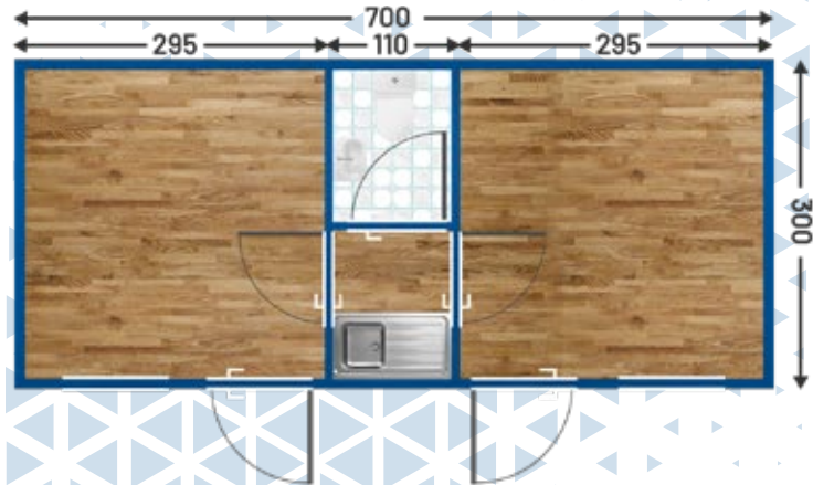
Model K-110
