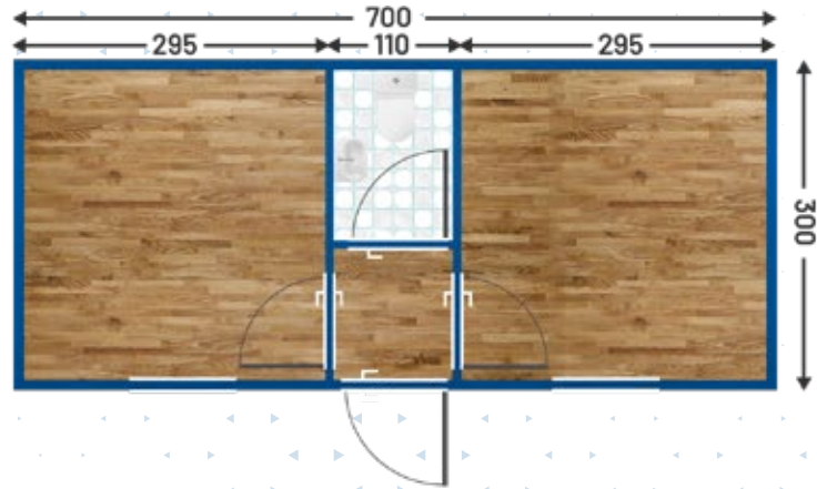
Model K-109
