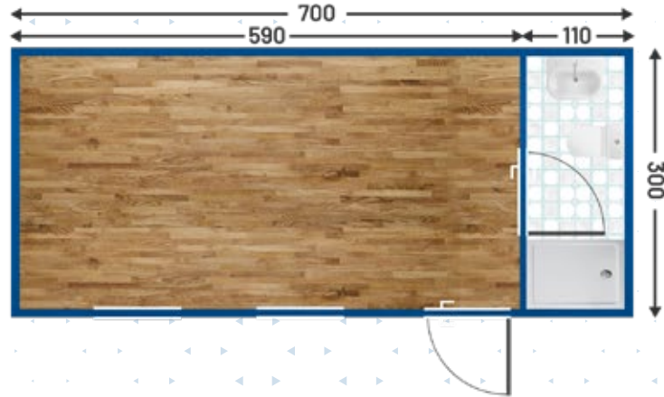
Model K-107
